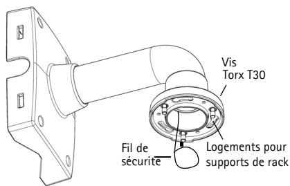
Support mural (exemple de fixation)
