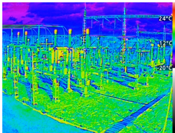
A similar scene as seen by an Axis thermometric camera. The camera detects and measures infrared radiation and converts the result to temperature readings. The different temperatures are also visualized using a color palette.
