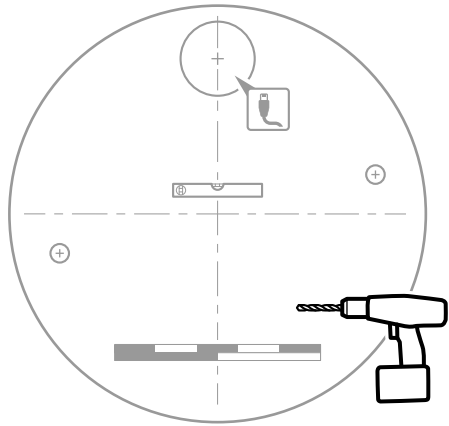
Drill template
