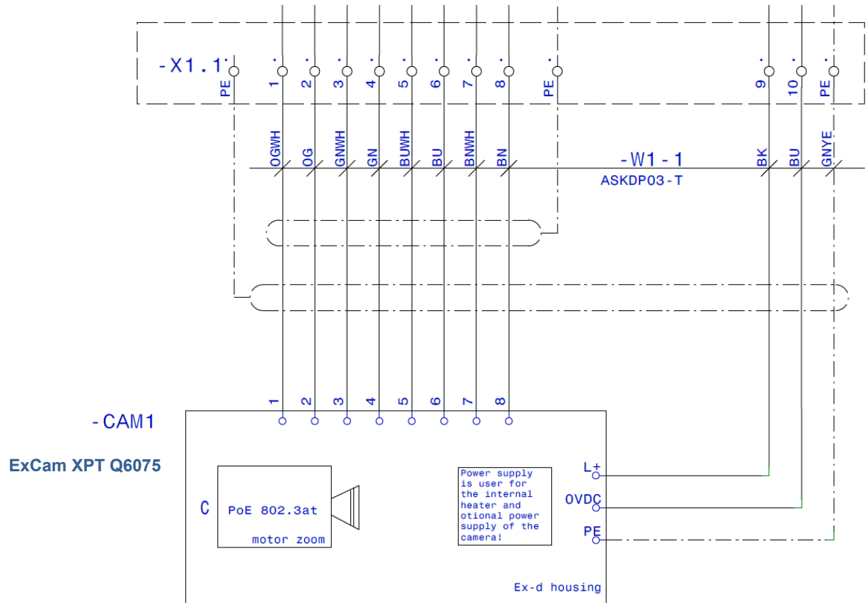
Fig. 5-4 Sample circuit of terminal box ExTB-3
