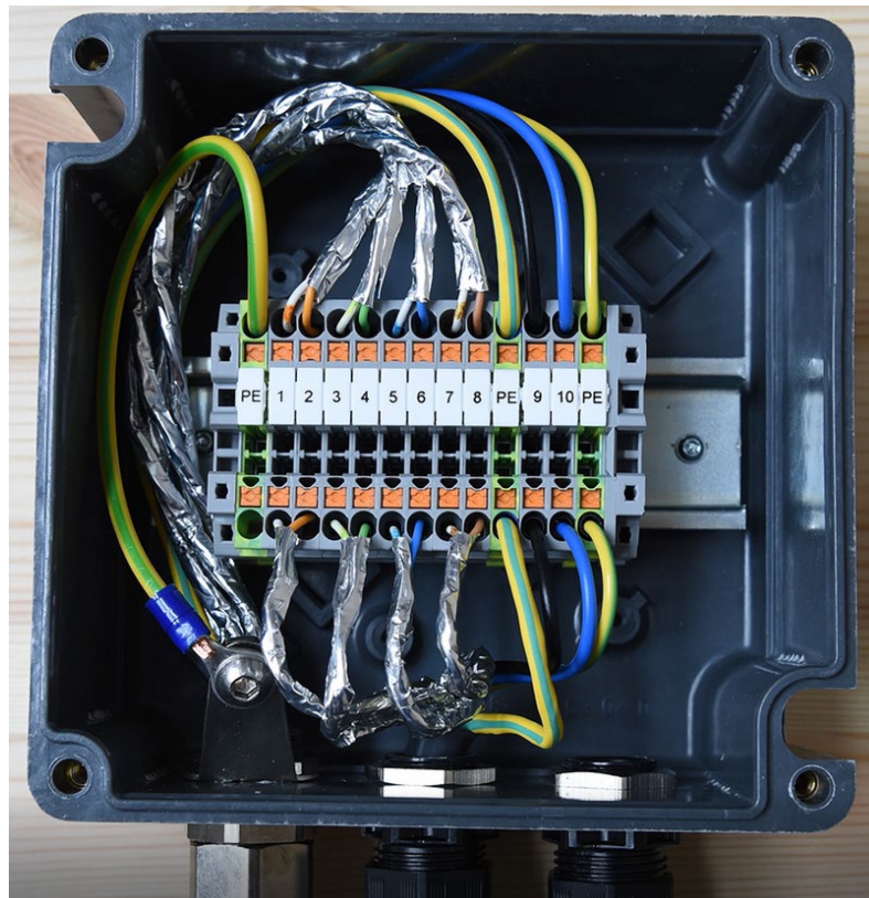
Fig. 5-5 Photo of the occupied terminal box ExTB-3
