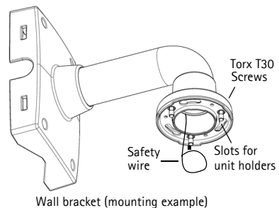
Wall bracket (mounting example)
