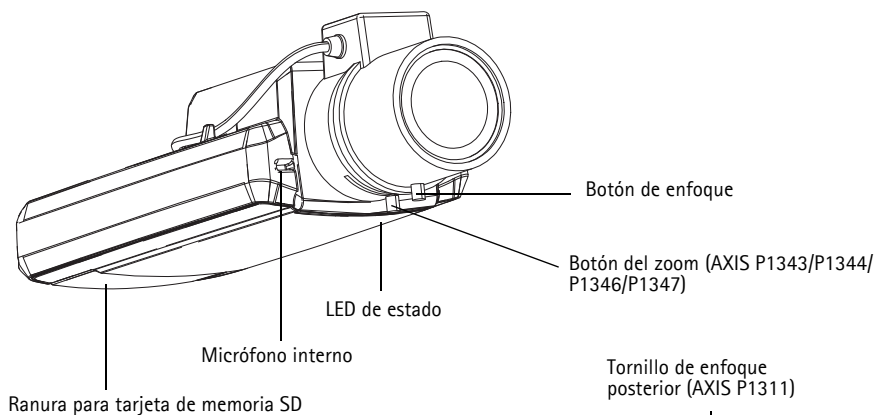
Vista superior – AXIS P1343
