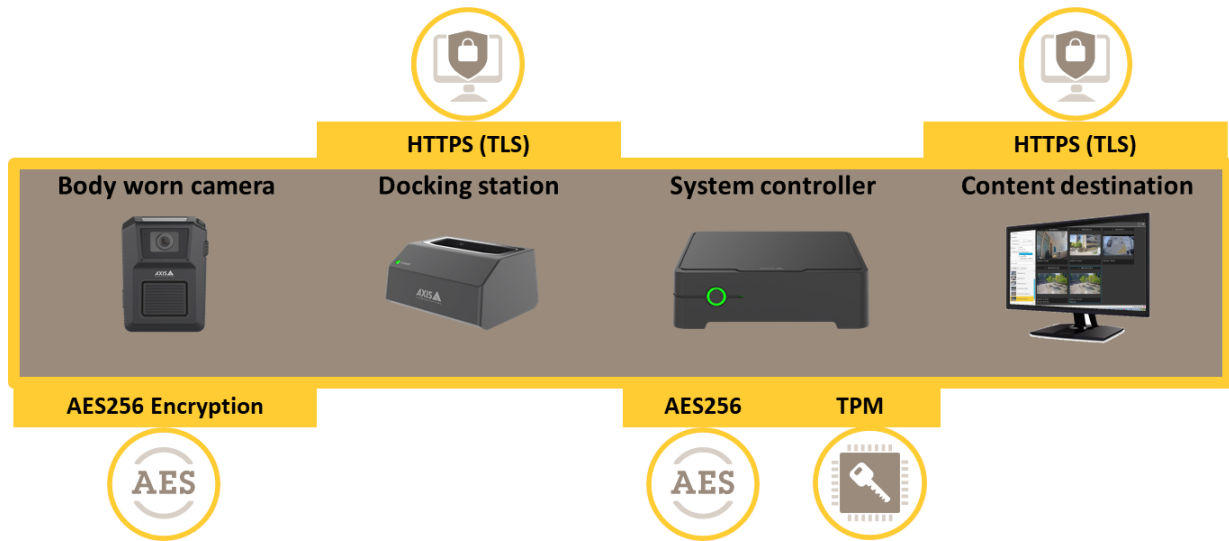
Figure 1. Secure data storage and data transfer from the BWC to the content destination.
