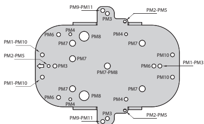
Moving plate
