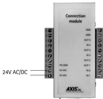
AXIS 231D+/232D+ Connection module
