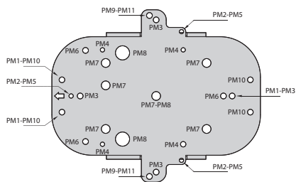
Piastra mobile
