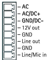
AXIS 233D Connector
