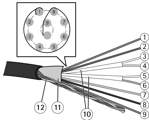
Multi-connector cable overview
