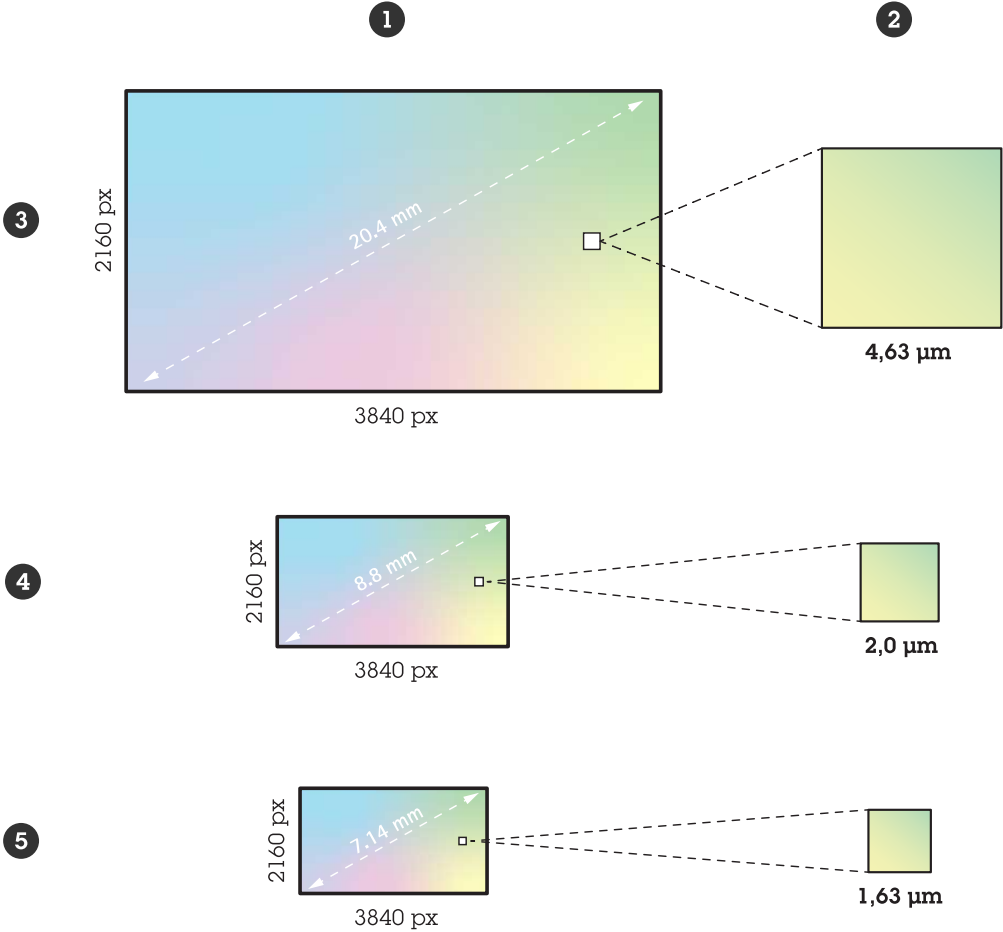
Figure 1. Comparing sensor sizes and pixel sizes between a selection of 4K network cameras. The sensor size and pixel size of Axis premium 4K cameras with large sensors are more than four times larger than those of typical or industry premium 4K cameras.
