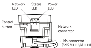
AXIS M1103/M1104
