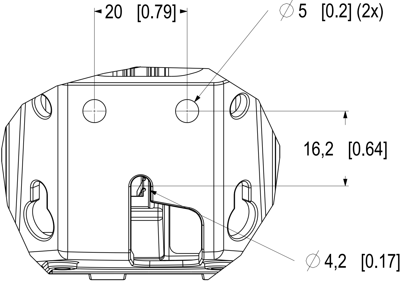
DETAIL B (2:1)
