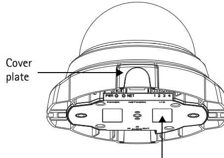
Dome casing for AXIS 212 PTZ-V
