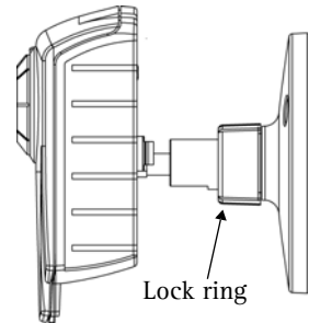
Wall mounting
