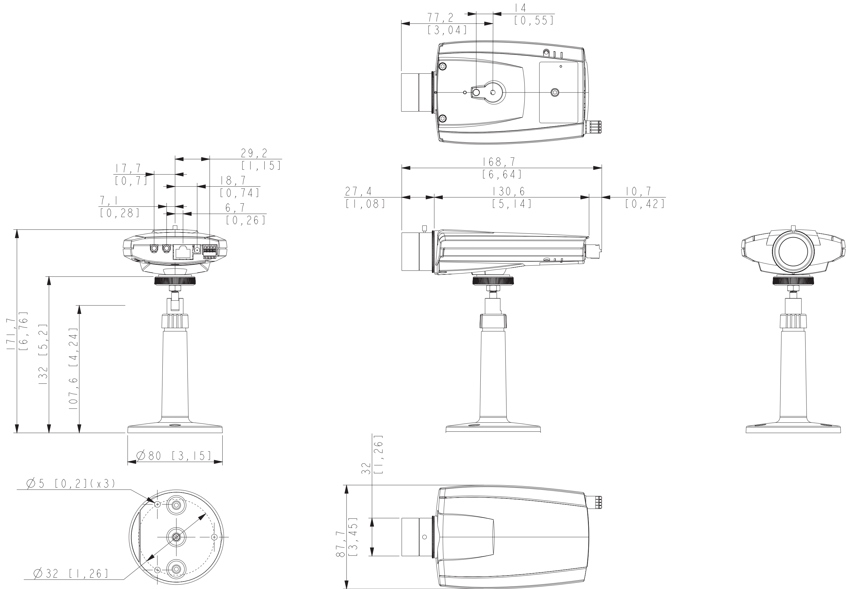
AXIS 210A - Network Camera 3 SEPT, 2007
